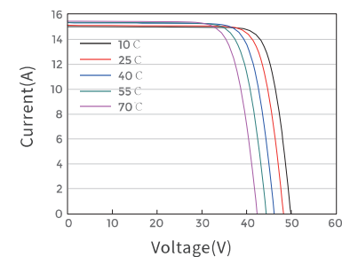
Current-Voltage Curve JAM66D42-580/MB/1500V Power-Voltage Curve JAM66D42-580/MB/1500V Current-Voltage Curve JAM66D42-580/MB/1500V
