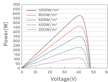
Current-Voltage Curve JAM66D42-580/MB/1500V Power-Voltage Curve JAM66D42-580/MB/1500V Current-Voltage Curve JAM66D42-580/MB/1500V
